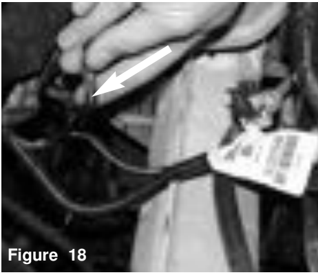
Figure 18 The electrical tape is removed exposing black and red wires that will be tucked into the wire loom.
