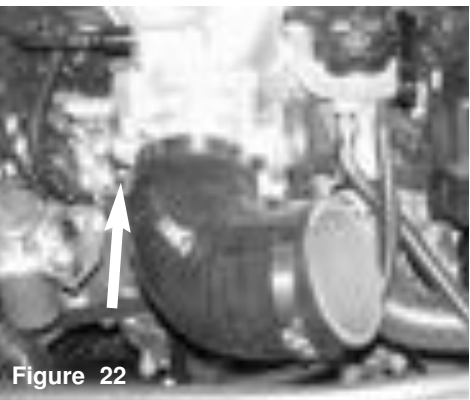
Figure 22 The 90 degree elbow is now resting over the throttle body, the clamp over the throttle body is semi-tightened.
