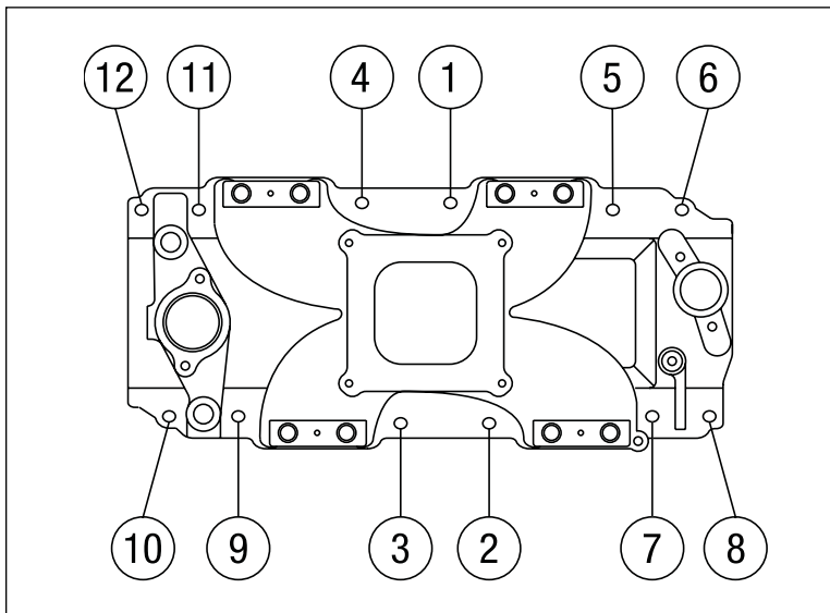
Figure 1 - Bolt tightening sequence, tighten bolts to 25 ft./lbs.
