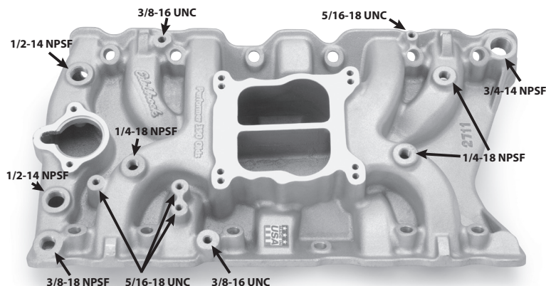
Fitting Boss Thread Sizes (Depending on application, not all bosses will be present)
